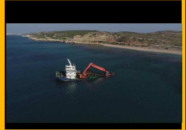
Operation for the Salvage of the KANUNIS
