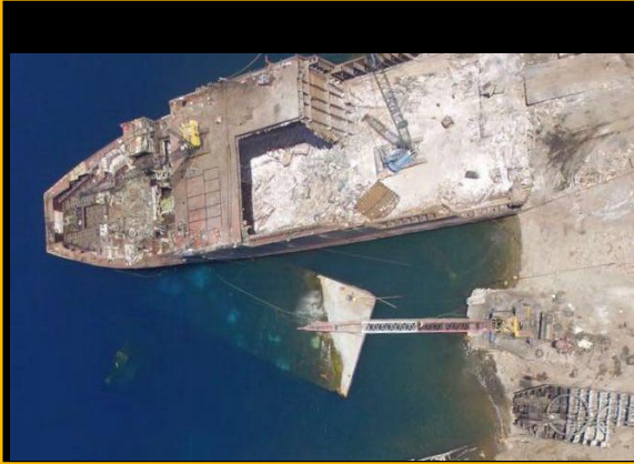
Recovery and Floating of 2000 Tonne ATLANTIS V Pontoon
